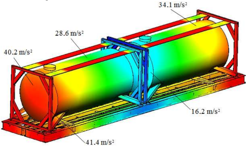
Figure 2.22 – Distributions of the accelerations to the flat car with tank containers during a shunting impact
