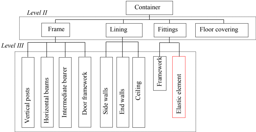
Figure 2.10 – Block-hierarchy diagram of a ICC dry-cargo container structure
