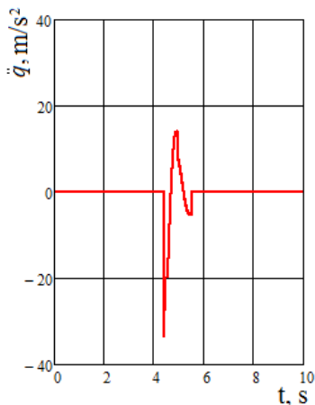
Figure 2.18 – Accelerations to a tank container with elastic-viscous links in the fittings, located on the flat car during a shunting impact
