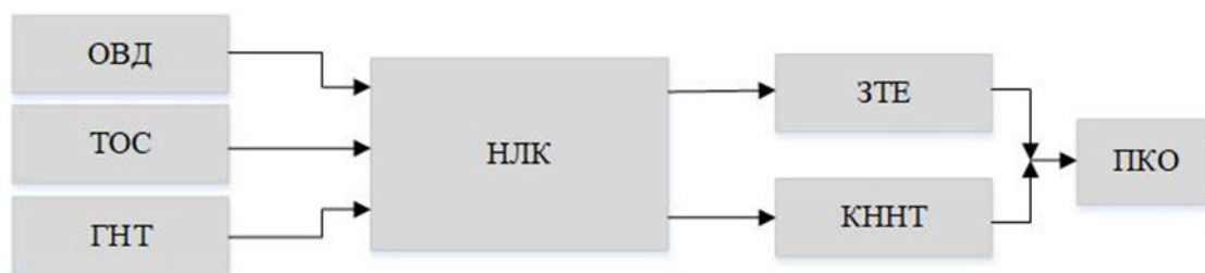
Figure 3. A block diagram of the transformer residual life monitoring device (In Ukr.)
