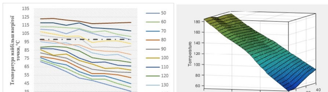
Figure 2. Dependence of the corresponding temperature value on the transformer load and ambient temperature (In Ukr.)
