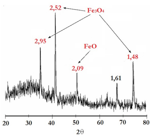
Figure 3. Diffraction pattern of composite glass No. 1
