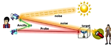
Quantum illumination
