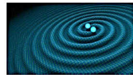
Squeezing and entanglement for gravity wave detectors
