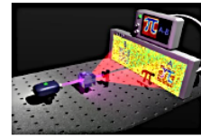
Sub-shot-noise imaging
