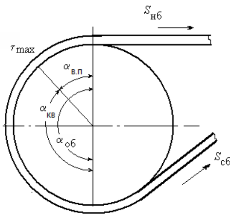
Figure 1. Scheme of determining the traction force transmitted by the drive drum of the belt conveyor
